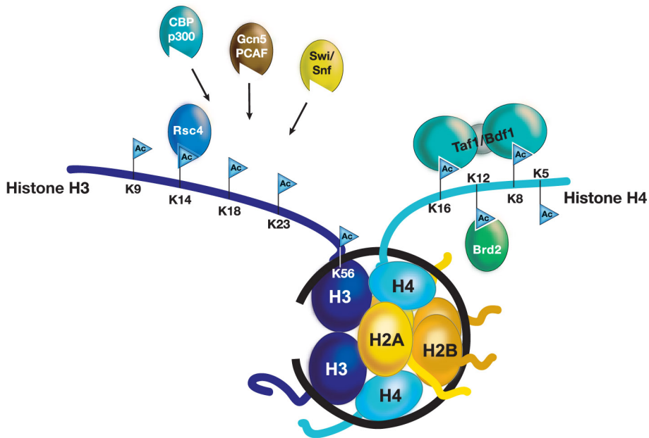
Figure 3. Characterized Sites of Histone Acetylation
