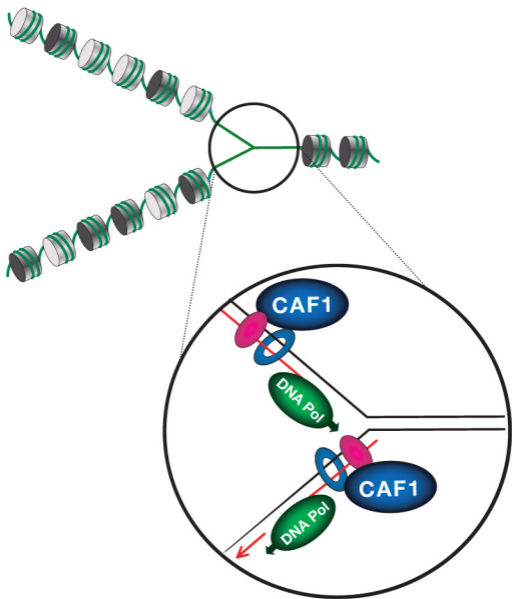
Figure 3. Old Nucleosomes ( dark disks ) Are Randomly Distributed behind the Replication Fork and New Nucleosomes ( light disks ) Are Deposited in the Gaps
